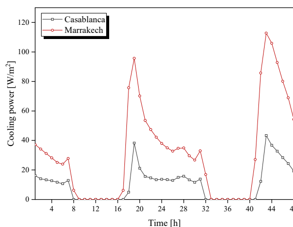
Fig. 6 Cooling power in Marrakech and Casablanca
