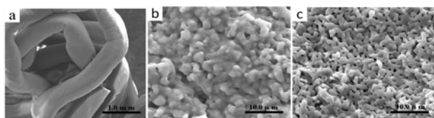
Fig. 4 SEM photographs of HA and CuHA scaffolds (a) the morphology of fibers in scaffolds (b). The HA scaffolds (c) and CuHA scaffolds (D)
