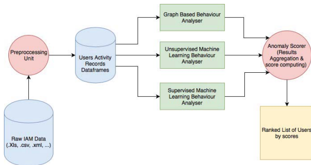
Fig. 1 Proposed Ensemble Learning Framework
