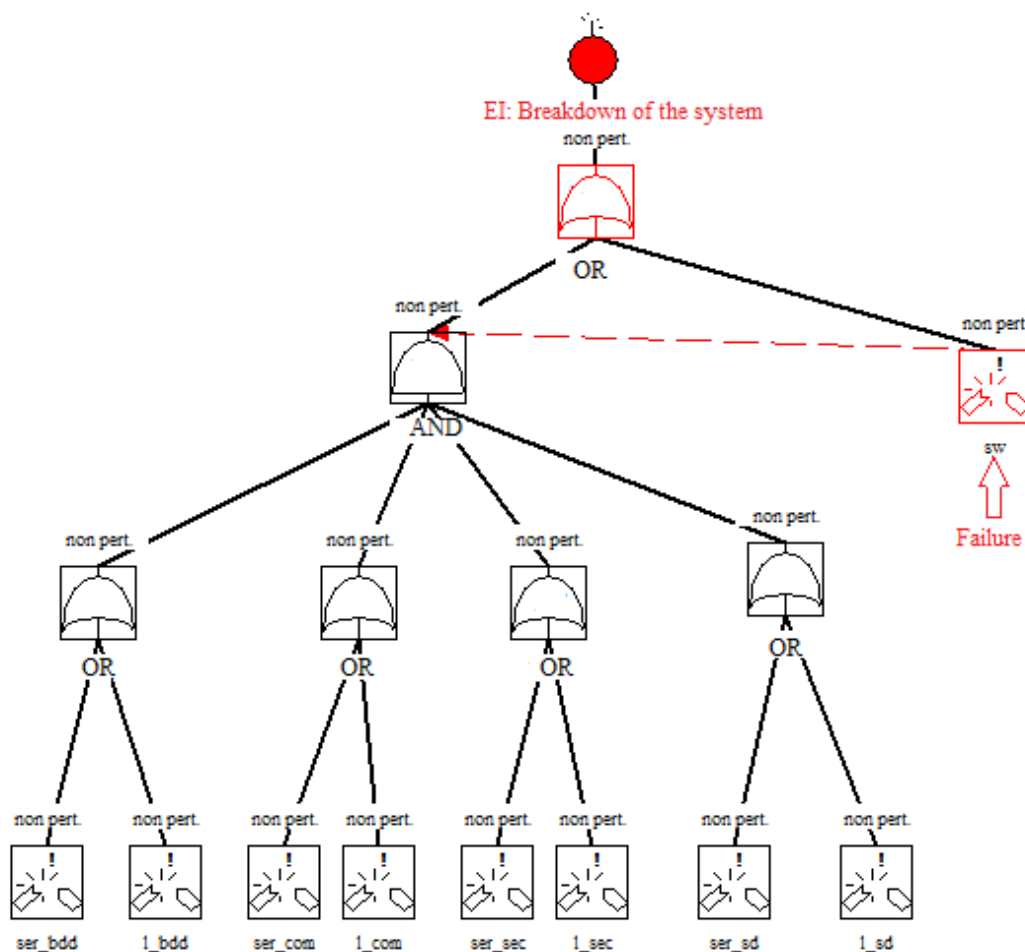
Fig. 7 Simulation of the system breakdown
