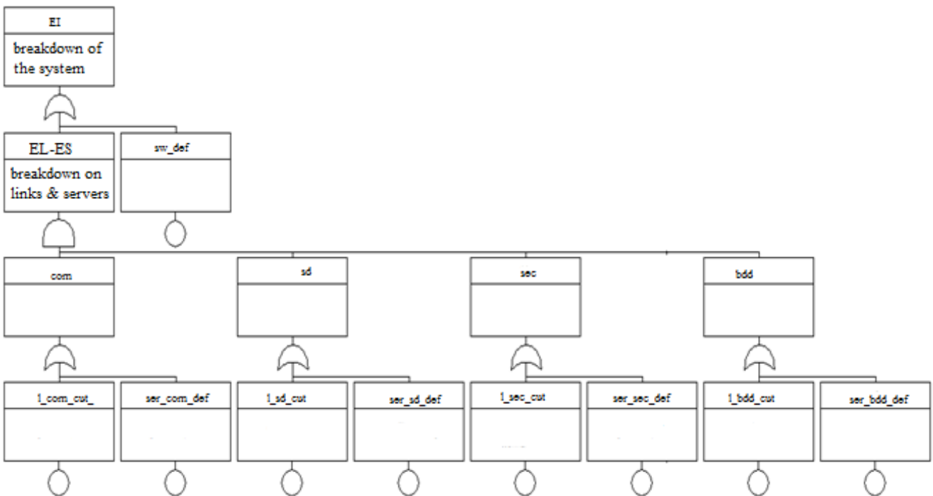
Fig. 6 BDMP of the network
