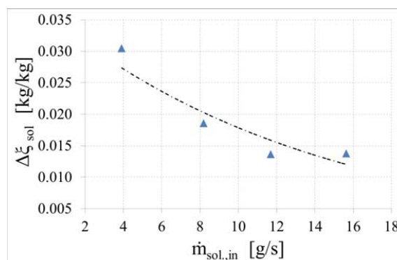
Fig. 7 Concentration spread as a function of solution mass flow rate
