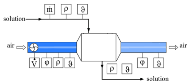
Fig. 5 The experimental setup of the absorber
