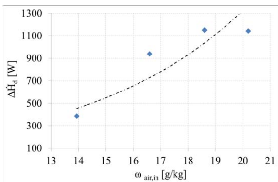
Fig.11 Dehumidification load as a function of humidity ratio
