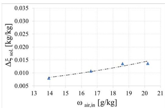
Fig. 10 Concentration spread as a function of humidity ratio
