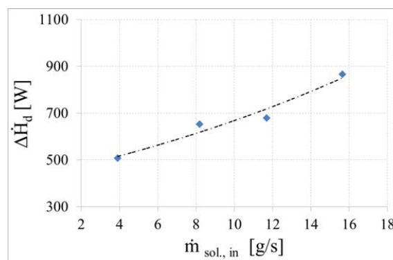
Fig. 8 Dehumidification load as a function of solution mass flow rate
