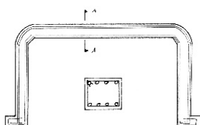
Fig. 9 Reinforcement of the original frame
