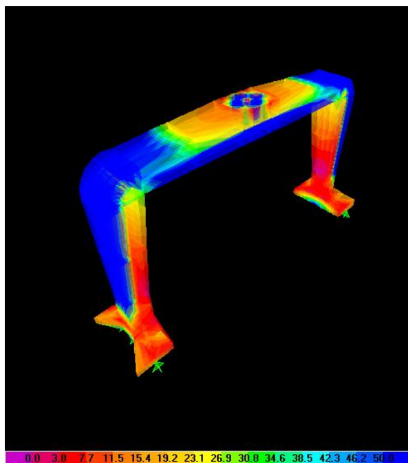
Fig. 15 Optimized frame model using SAP software
