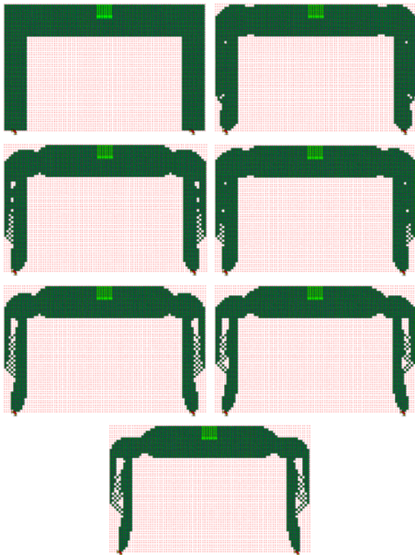
Fig. 13 Display the stages of geometric frame optimization
