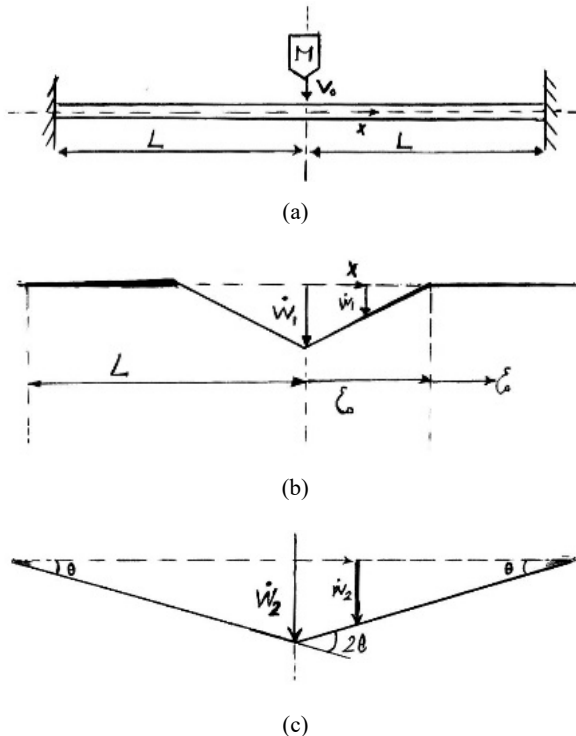
Fig. 7 (a) Stroke of mass (M) with initial velocity of V with fixed beam, (b) Index of transverse velocity for first phase of motion, 0 \leq t \leq t_1 , (c) Index of transverse velocity for second phase of motion t_1 \leq t \leq T
