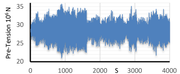
Fig. 2 Response of the tether 1 before failure in sea state S 1
