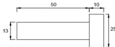
(b) Shape and size of stud (unit: mm)
