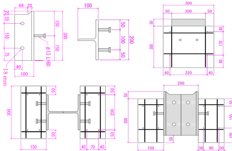
Fig. 3 Pushout test specimen details
