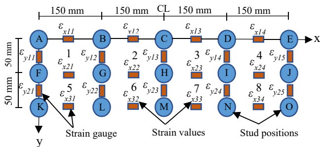
(b) Detailing of element and nodal studs
