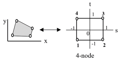
Fig. 8 Shape function
