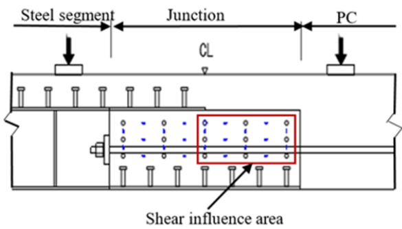
Fig. 11 Shear influence area
