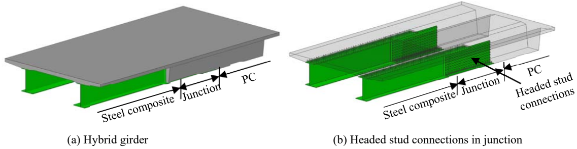
Fig. 1 Hybrid girder and junction
