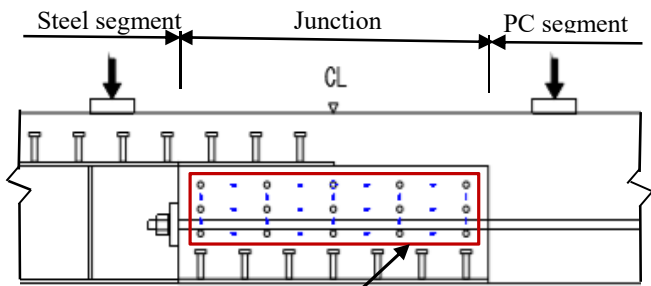
Stud and strain gauge positions in web (a) Stud and strain gauges positions in web
