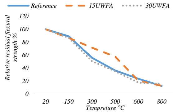
Fig. 8 Relative residual flexural strengths as a function of temperature of SCC incorporated UWFA up to 30% as a replacement of cement
