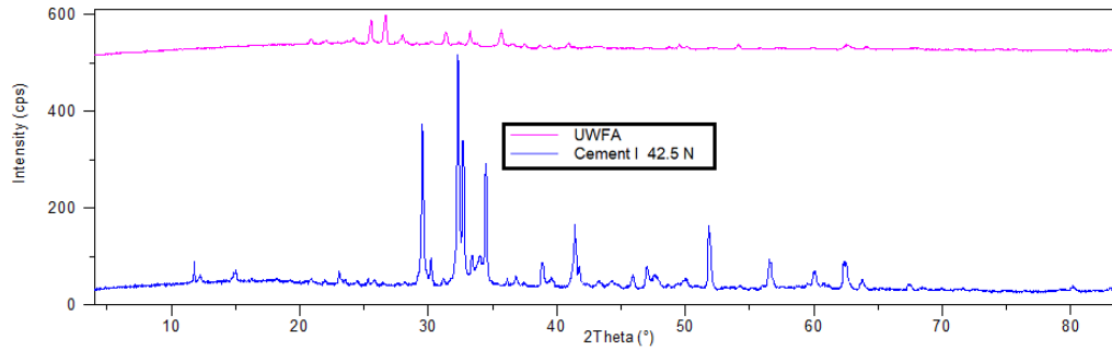
Fig. 1 X-ray diffraction profile for cement and UWFA
