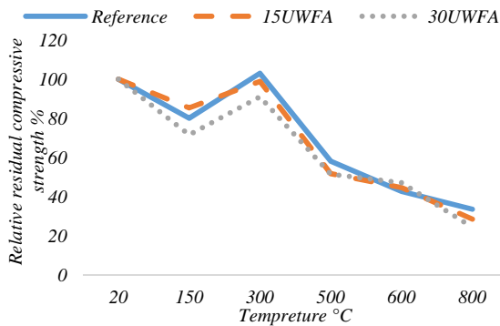
Fig. 7 Relative residual compressive strengths as a function of temperature of SCC incorporated UWFA up to 30% as a replacement of cement
