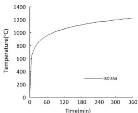
Fig. 5 ISO-834 fire curve
