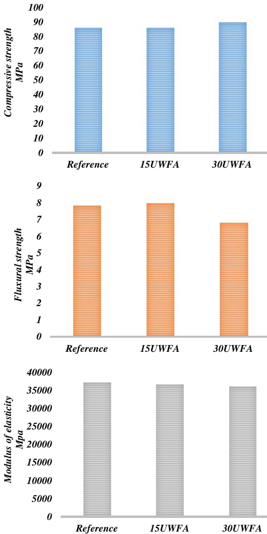
Fig. 6 Compressive strength, flexural strength and modulus of elasticity at laboratory temperature (90 days)
