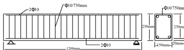
Fig. 3 Specimen details
