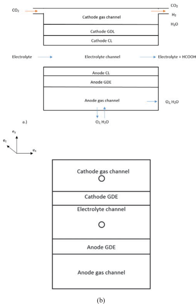
Fig. 1 Schematics of (a) the front and (b) the side view of a microfluidic electrochemical cell
