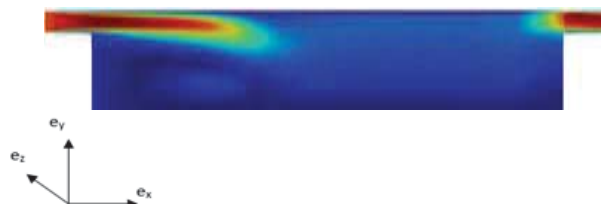
Fig. 3 Concentration contour of CO 2 in gas channel (mol/m 3 ): mole ratio 0.5:0.5 Bi-Sn particle catalyst;
