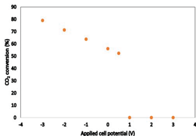
Fig. 6 CO 2 conversion versus applied potential using [EMIM][BF 4 ]
