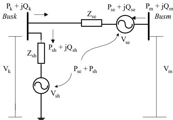
Fig. 3 UPFC Equivalent Circuit
