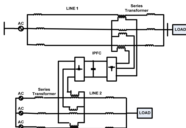
Fig. 1 Schematic diagram of IPFC
