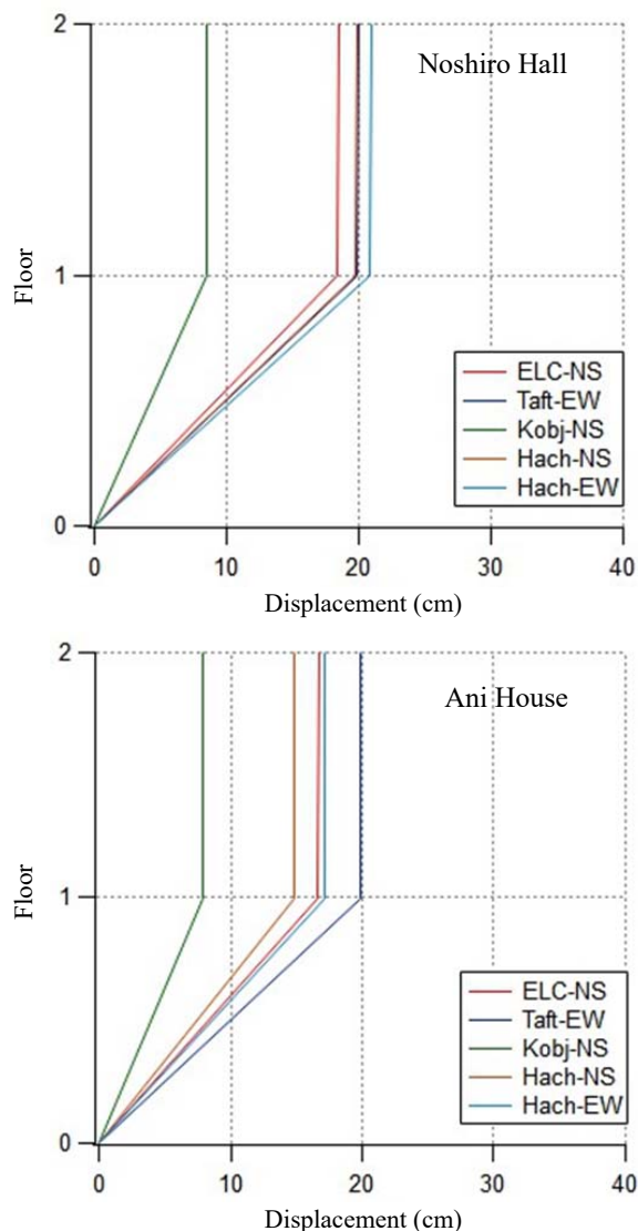
Fig. 9 Maximum displacement responses of target buildings
