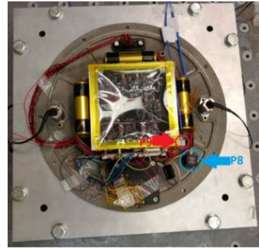
Fig. 8 DOC- P8-P9 Measurements Accelerometers location
