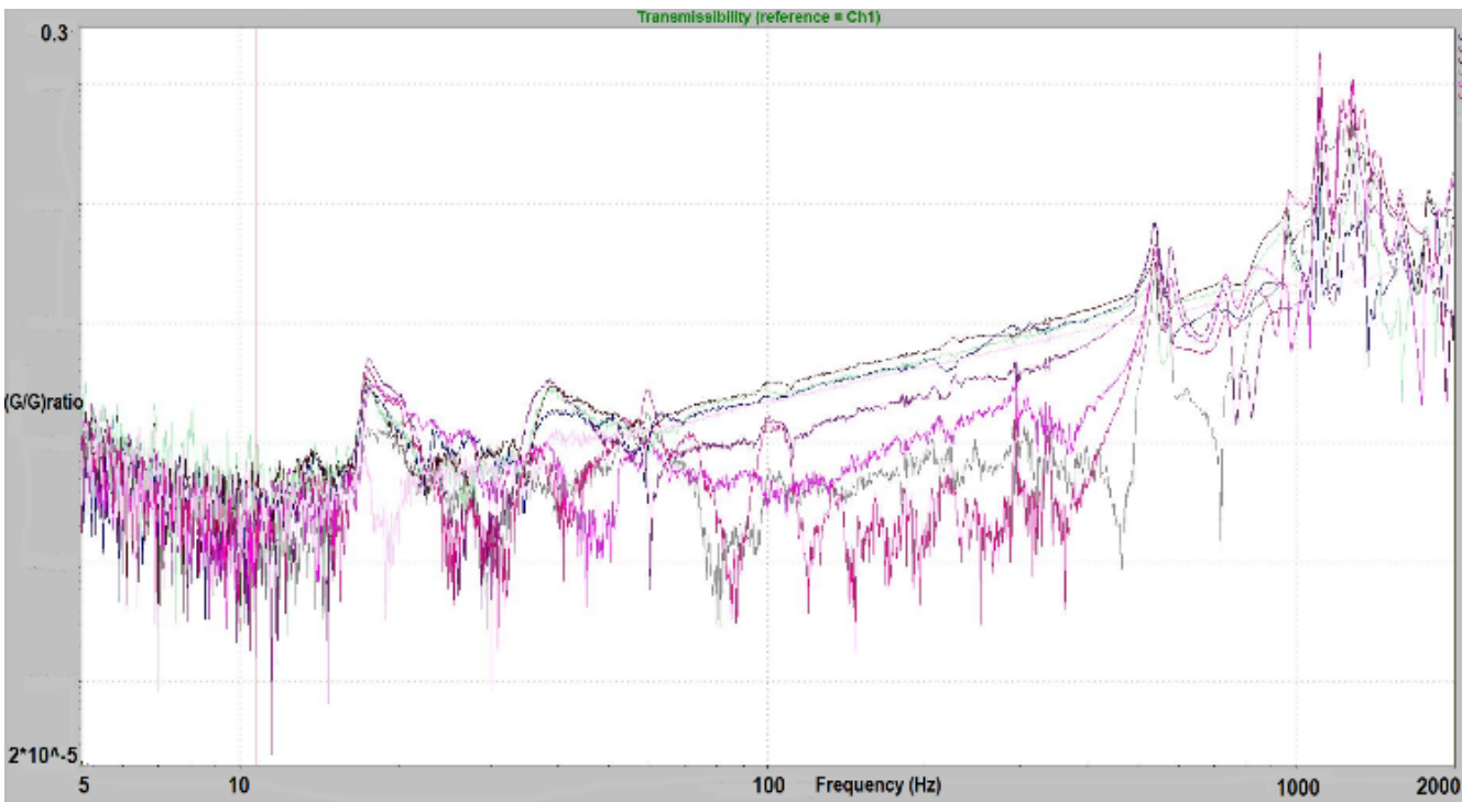
Fig. 5 Fixture Experimental Resonance Search
