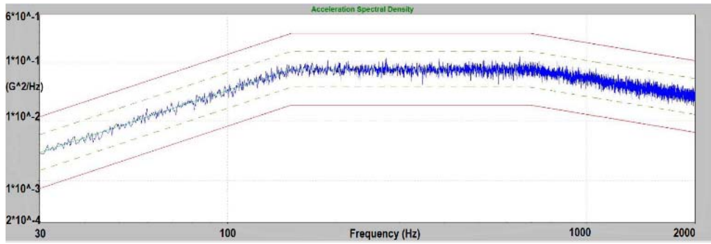
Fig. 12 DOC EQM Power Spectral Density –Measured Levels
