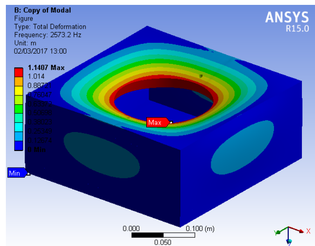
Fig. 3 Fixture FEM model
