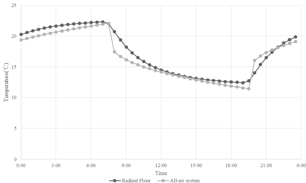
Fig. 6 Ceiling Temperature of RF and AA System
