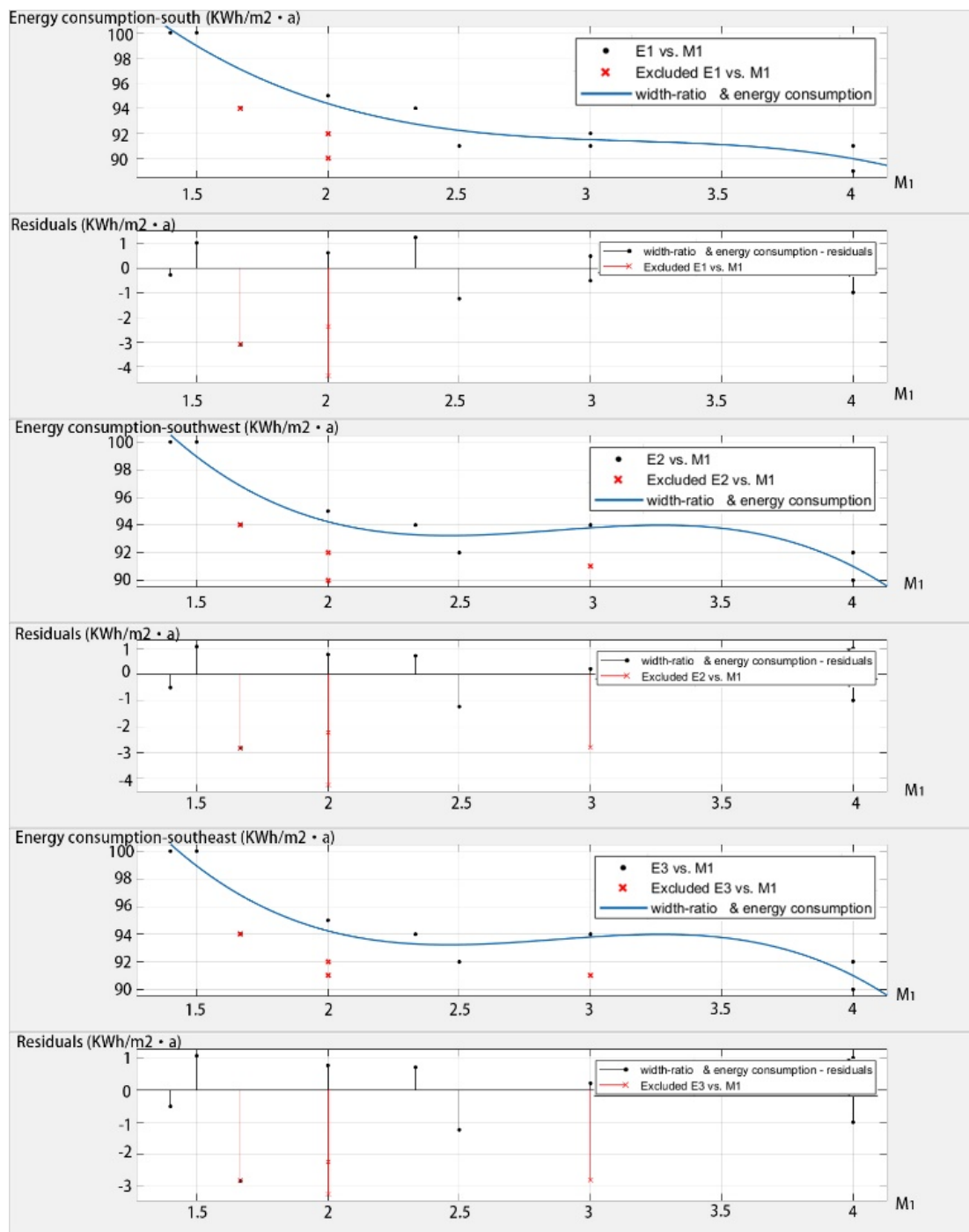
Fig. 8 Regression fitting of width-ratio and energy consumption of buildings
