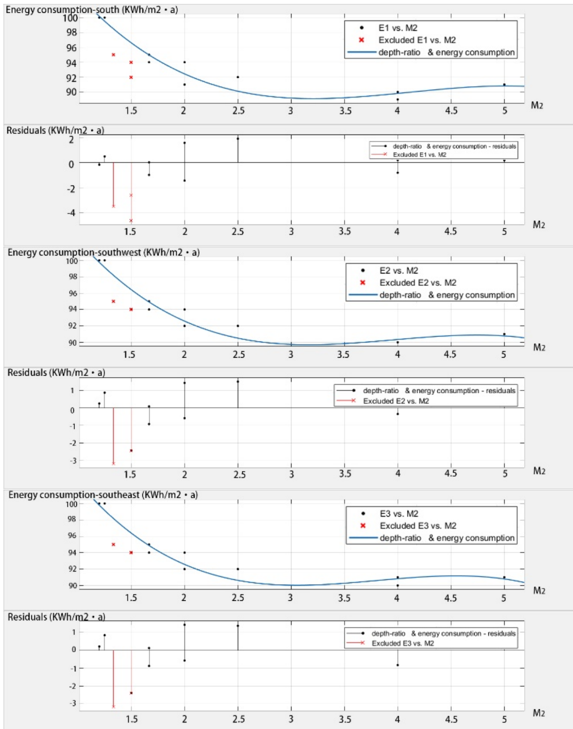
Fig. 9 Regression fitting of depth-ratio and energy consumption of buildings
