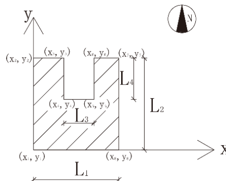
Fig. 1 Diagram of parametric model of U-shaped buildings
