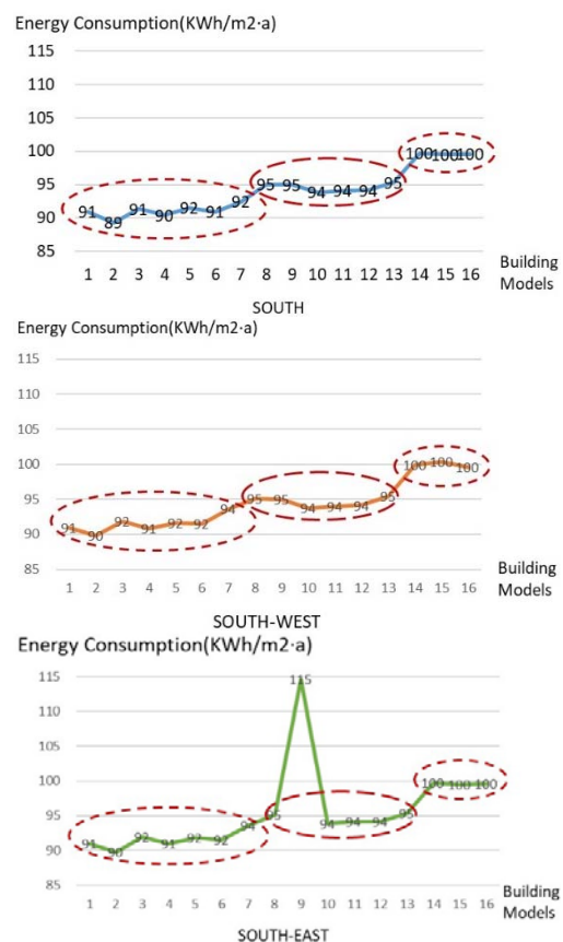
Fig. 7 The relationship between layouts and energy consumption in different building orientation
