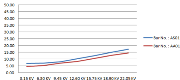
Fig. 10 Tan delta trend of AA01 & AS01
