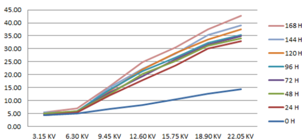
Fig. 9 Tan delta trend of AA01 (RR system)
