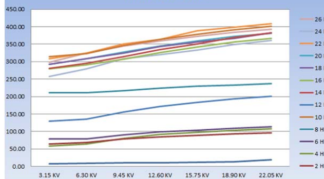
Fig. 11 Tan delta trend of AS01 (thermal & electrical stress)
