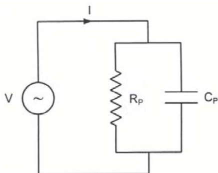
Fig. 4 Parallel circuit of resistor and capacitor
