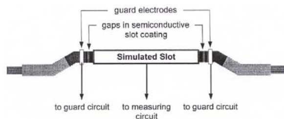
Fig. 6 Schematic of dissipation factor measurement on stator bar
