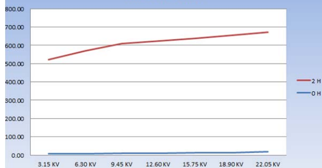
Fig. 12 Tan delta trend of AA01 (thermal & electrical stress)
