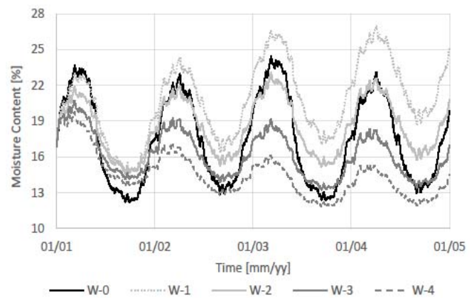
Fig. 5 OSB moisture content (Assembly 1)
