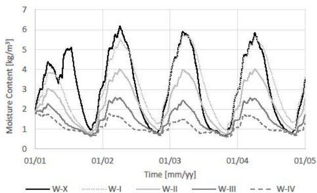
Fig. 7 Cavity moisture content (Assembly 2)
