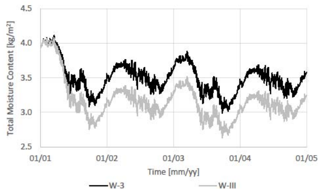
Fig. 9 Total moisture accumulation per square meter of a wall
