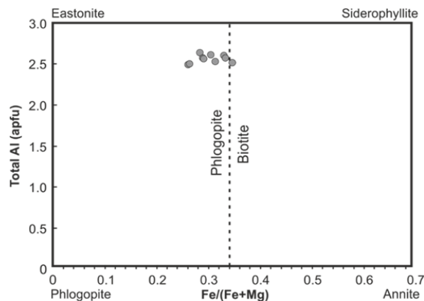
Fig. 2 Classification of biotite based on [16].
