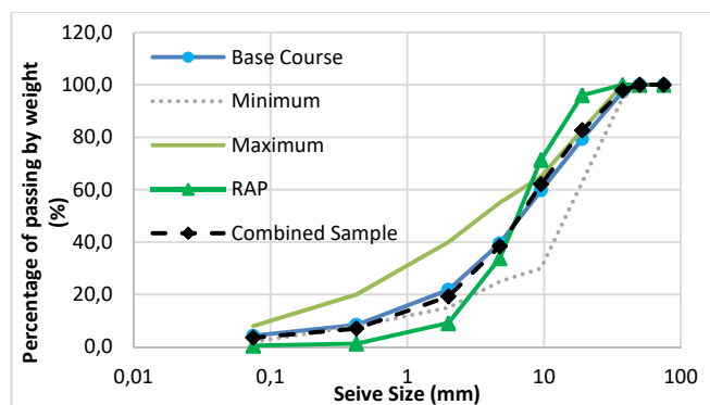
Fig. 7 Combined Sample according to the gradation specifications
