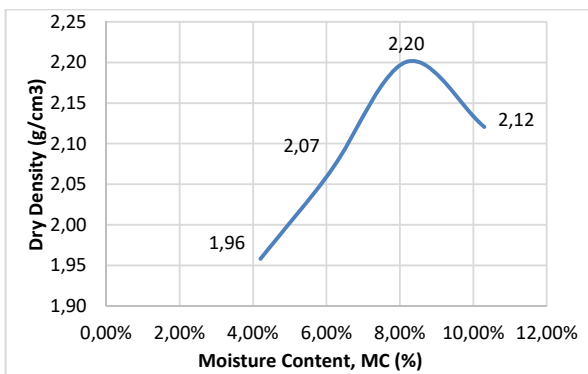
Fig. 5 Modified Proctor test results
