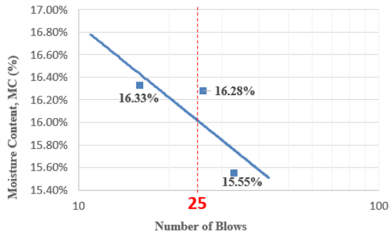
Fig. 4 Moisture Content vs. Number of Blows
