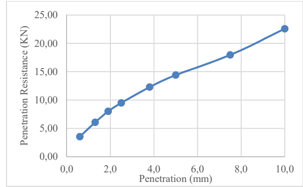
Fig. 6 Penetration Resistance vs. Penetration Rate during CBR Test
