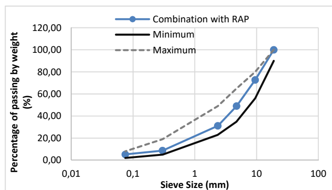
Fig. 8 New Asphalt Formula (Aggregates+30% RAP) Sieve results
