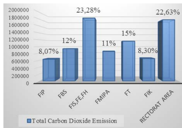
Fig. 1 Percentage Carbon Dioxide Emissions at UNNES
