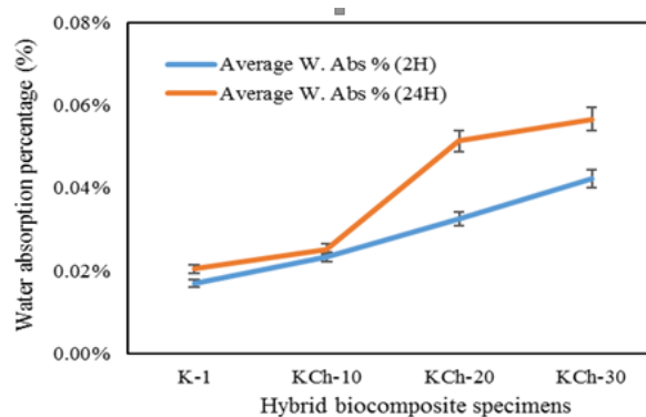
Fig. 2 Water absorption of hybrid bio-composite specimens
