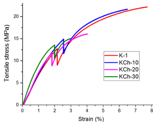
Fig. 3 Typical stress-strain curves of hybrid bio-composite specimens
