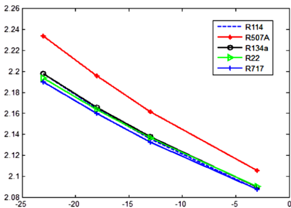
Fig. 2 The exergy destruction of various refrigerants with condenser temperature of 30°C
