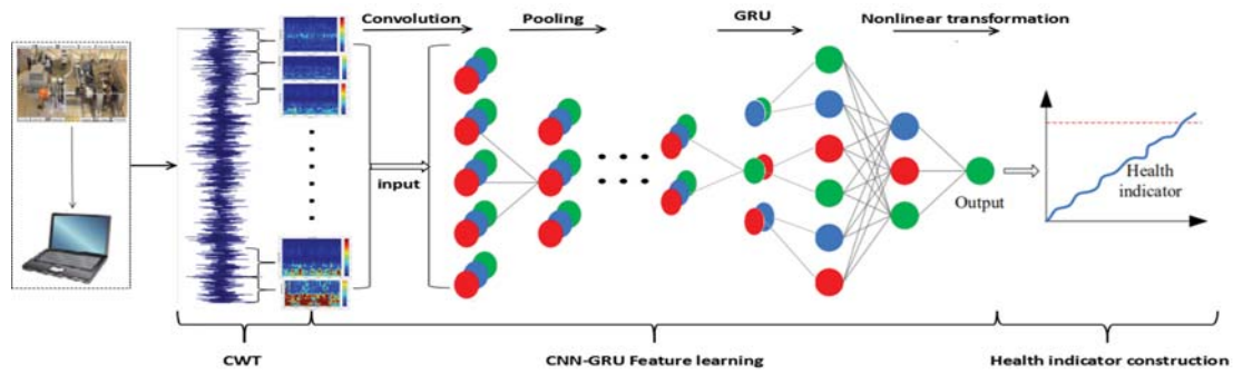
Fig. 3 The proposed CCG-HI model
