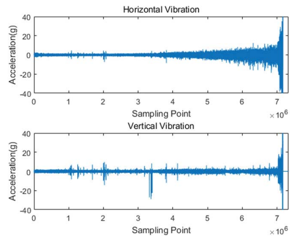
Fig. 5 The temporal vibration signal of bearing1_1
