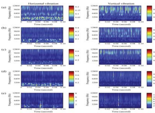
Fig. 7 TFRs of bearing1_1, where (a)-(e) refer to the 2000 th , 1500 th , 1000 th , 500 th and 1 th
