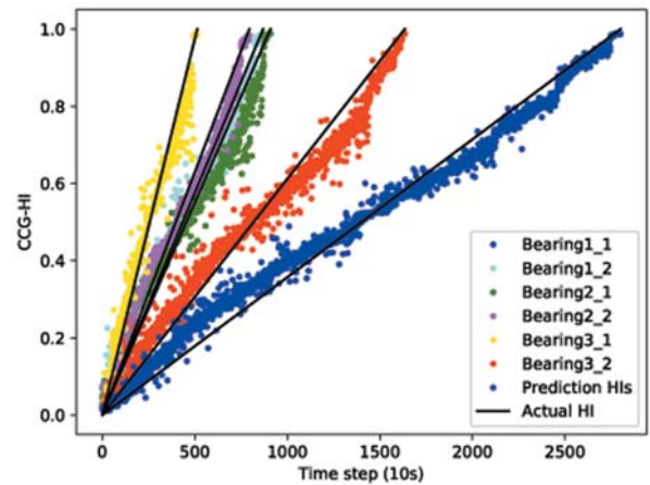
Fig. 8 CCG-HI of the six training datasets
