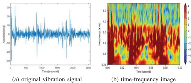
Fig. 2 Signal-to-image of Bearing1_1 at 28000 s
