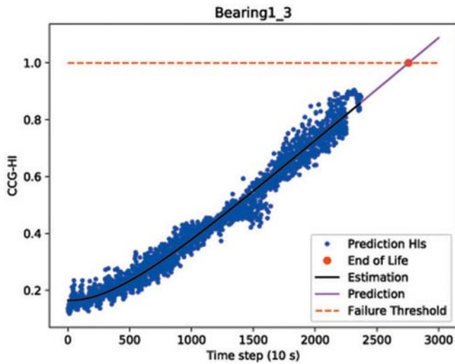
Fig. 10 RUL prediction result of bearing1_3
