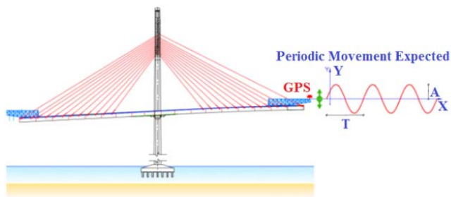
Fig. 1 Simulation of vibration during the process of construction
