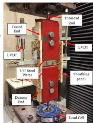
Fig. 6 Nail joint test setup
