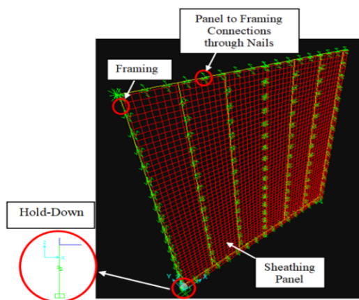
Fig. 8 Shear wall model in SAP 2000
