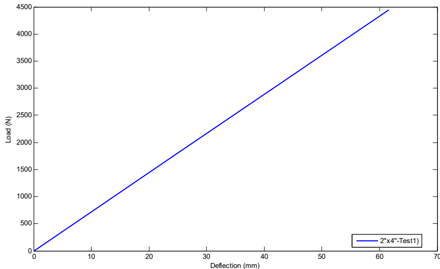
Fig. 4 2x4 Stud typical bending performance
