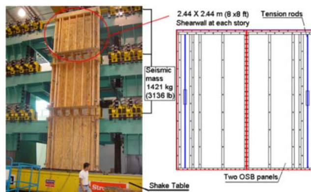
Fig. 1 3-storey shear wall test configuration [5]
