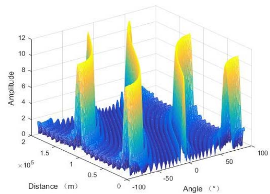
Fig. 3 Three-dimensional view of the beam pattern (ULA-FDA)
