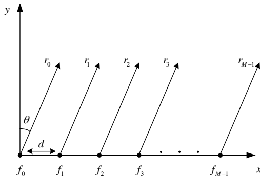
Fig. 1 Uniform linear frequency diverse array (ULA-FDA) structure
