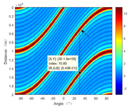
Fig. 4 Two-dimensional plane beam pattern (ULA-FDA)
