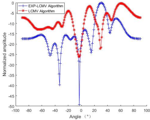
Fig. 10 Comparison of LCMV algorithm and EXP-LCMV algorithm beam pattern (angle dimension)
