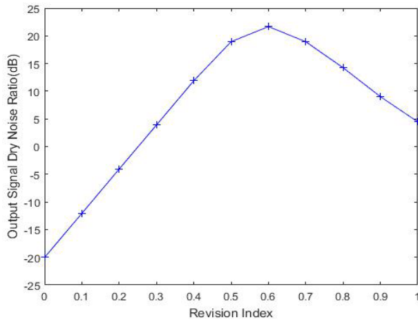
Fig. 13 Output SINR changes with correction index
