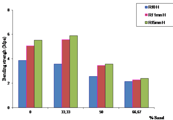
Fig. 7 Bending strength of plaster mortars
