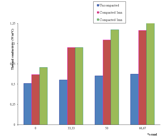
Fig. 9 Thermal conductivity of various plaster mortars at different times of compaction
