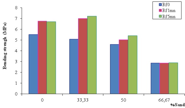
Fig. 5 Bending strength of dry plaster mortar
