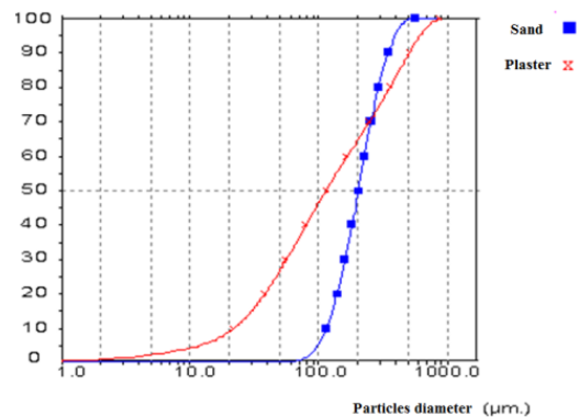
Fig. 1 Grain size curves of the used plaster and sand
