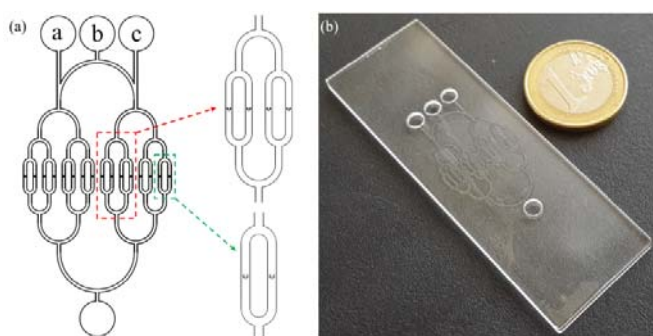
Fig. 2 (a) Design of the microfluidic device (a, b and c can be used as yeast or medium inlets) (b) Fabricated microfluidic device
