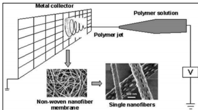
Fig. 1 Schematic diagram for the electrospinning process [7]
