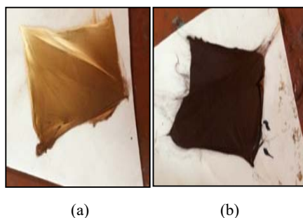
Fig. 4 Stabilized PAN fibers at 700 0 C for (a) Flat plate collector (b) Drum plate collector
