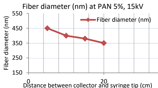
Fig. 8 Effect of separation between syringe head and collector on fiber diameter
