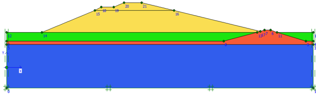
Fig. 1 Modeling of the present problem in PLAXIS
