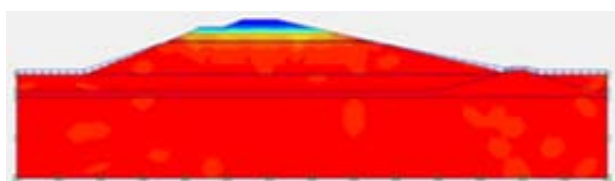
Fig. 6 Degree of saturation
