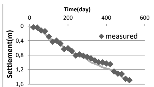
Fig. 8 Settlement versus time implemented with numerical solution
