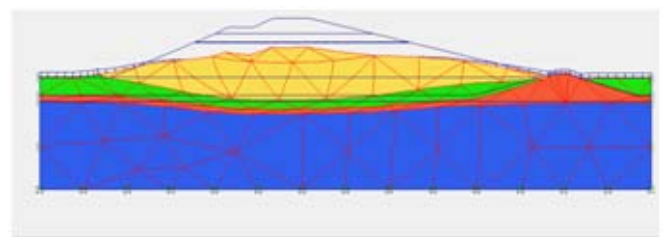
Fig. 5 Deformed mesh in phase 6
