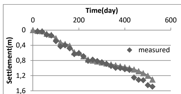
Fig. 7 Settlement versus time implemented with PLASIX
