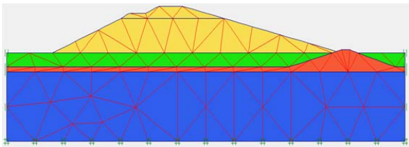
Fig. 2 Mesh of the present embankment in PLAXIS
