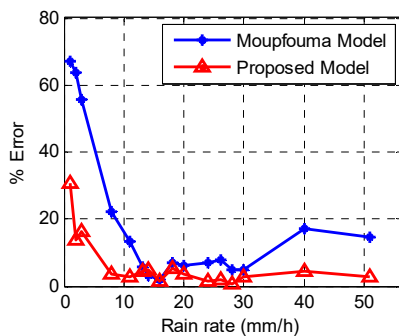
Fig. 11 Prediction errors for Moupfouma and proposed cell ratio model at 19.5 GHz
