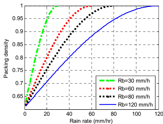
Fig. 3 Variation of rain drop packing density with rain rate of various R_b
