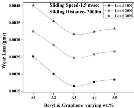
Fig. 8 Effect of load on heat treated composites
