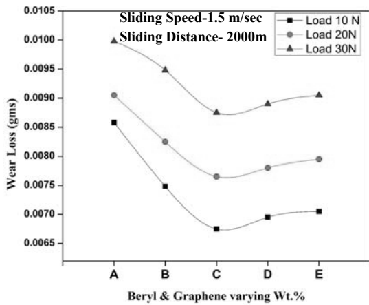
Fig. 7 Effect of load on as cast composites
