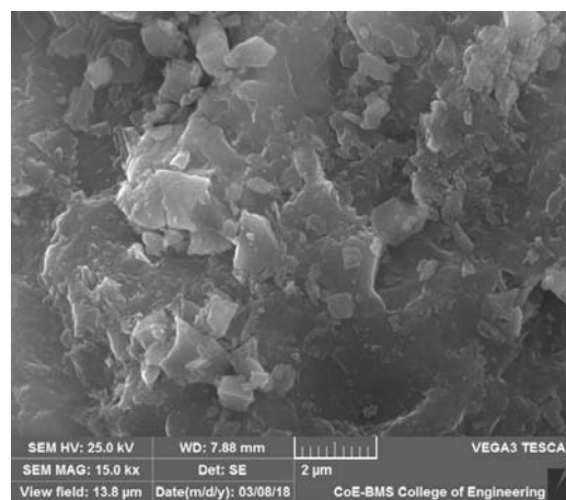
Fig. 1 SEM image of beryl particles
