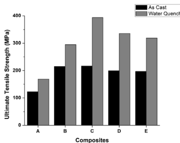
Fig. 6 Effect of heat treatment on ultimate tensile strength of Al7075 alloy and its composites in as-cast and solutionized conditions
