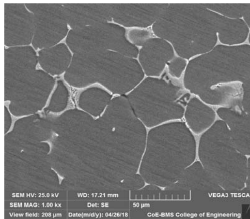
Fig. 4 (a) SEM image of Al7075 alloy
