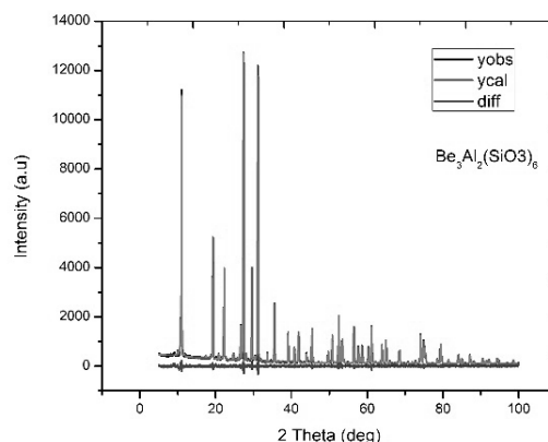
Fig. 2 XRD image of beryl particles
