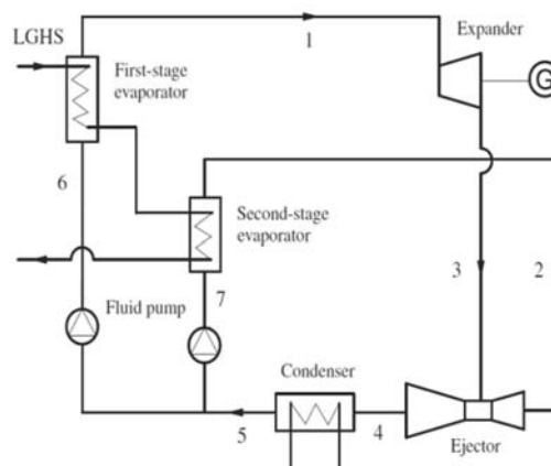
Fig. 3 Configuration and processes of the EORC
