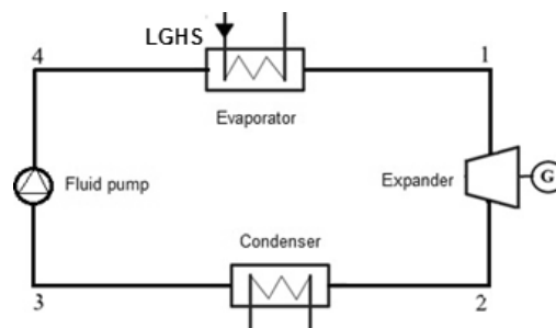
Fig. 1 The ORC configuration and processes
