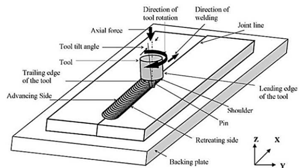
Fig. 1 Schematic drawing of FSW process
