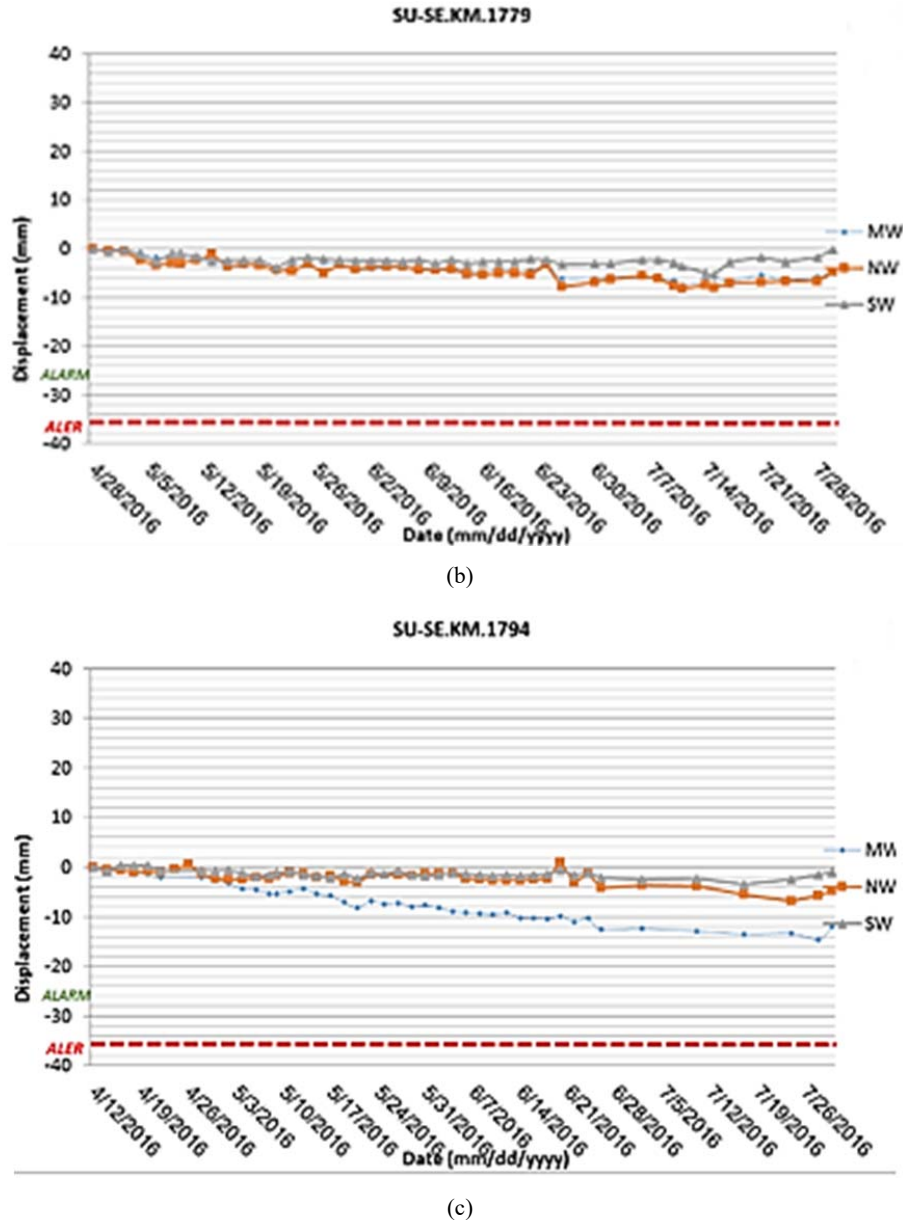
Fig. 10 The settlement readings of the top surface of the tunnel for three stages
