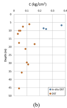
Fig. 13 The variations of shear strength parameters vs. depth of soil sample based on in-situ DST and laboratory DST; (a) internal friction angle, (b) cohesion
