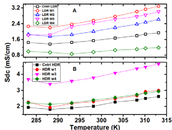
Fig. 3 Direct current conductivity, Sdc, as a function of temperature and time for LDR group (A) and HDR group (B)
