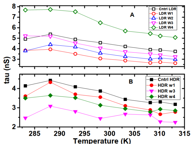
Fig. 2 Relaxation time as a function of temperature and time for LDR group (A) and HDR group (B)
