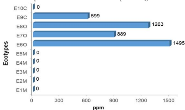
Fig. 6 Concentration of phorbol esters in the Jatropha curcas oil according to toxicity analysis
