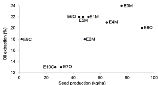
Fig. 5 Net seed oil Content calculated as the relation between seed production and oil extraction percentage
