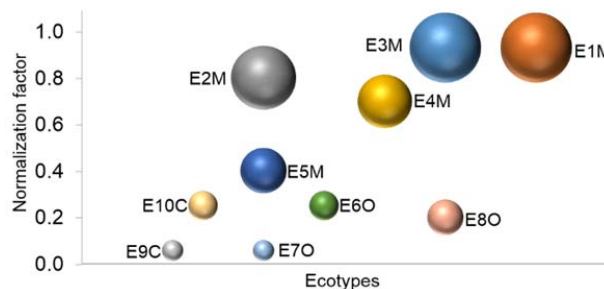
Fig. 7 Comparison of the normalization value of 10 ecotypes of Jatropha curcas
