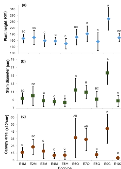
Fig. 3 Variation in biophysical parameters (mean±SD) at the end of the study (52 nd month) for 10 ecotypes of Jatropha curcas : (a) Plant height; (b) Stem diameter; (c) Canopy area. Values according to Tukey test A = higher growth, AB = high growth, B = medium growth, BC = low growth, C= lower growth. Same letters mean they are not significantly different ( p \leq 0.05 )
