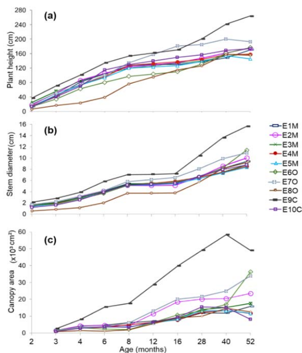
Fig. 2 Growth evaluation of 10 ecotypes of Jatropha curcas (C= Michoacán, M= Morelos and O= Oaxaca) by means of biophysical parameters at different plant ages in the plantation. (a) Plant height; (b) Stem diameter; (c) Canopy area
