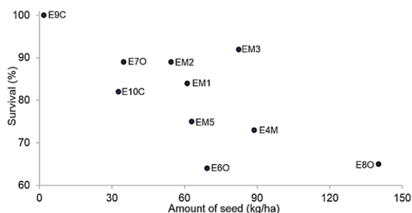
Fig. 4 Seed collected and Survival percentage at the experimental site by the end of the 52 nd month. The product of the multiplication of these parameters is the seed production
