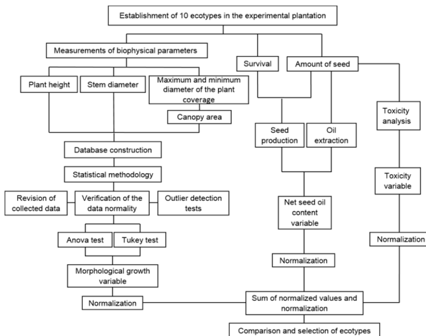
Fig. 1 Methodology evaluation of 10 ecotypes of Jatropha curcas in the experimental plantation
