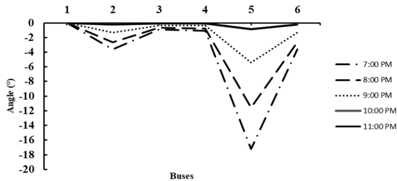
Fig. 13 Angle profile on bus 5 for a typical day
