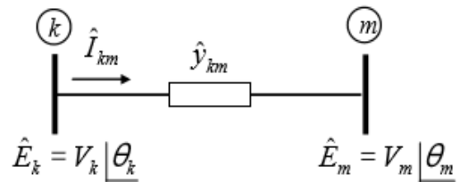
Fig. 3 Generic branch k - m for the calculation of losses
