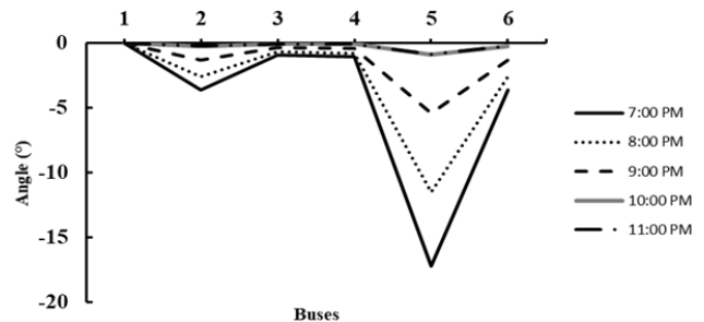
Fig. 15 Angle profile on bus 5 with generator and storage unit
