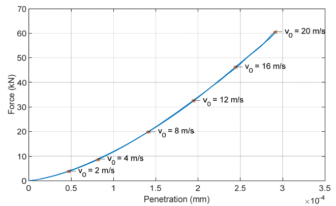
Fig. 5 Contact force versus penetration (elastic simulation)
