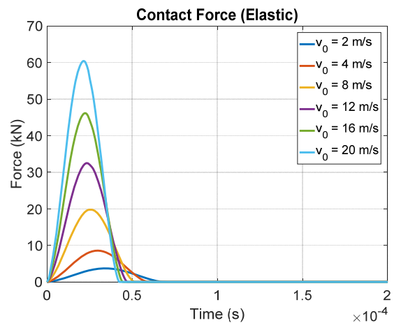
Fig. 3 Contact force for elastic model
