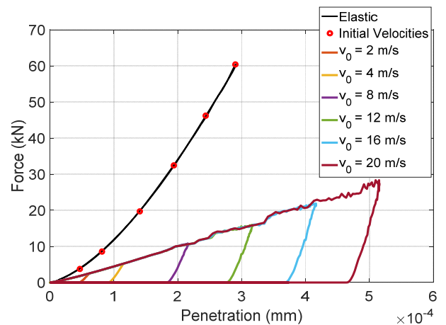
Fig. 9 Comparison contact force versus penetration (elastic simulation)
