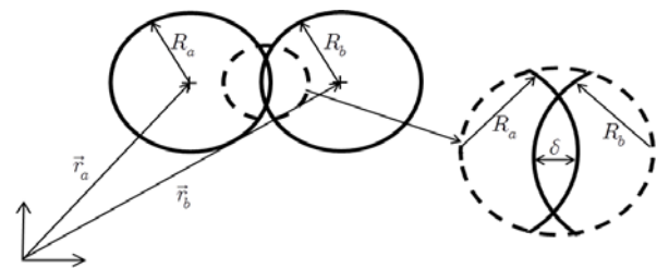
Fig. 1 Overlapping spheres with detail
