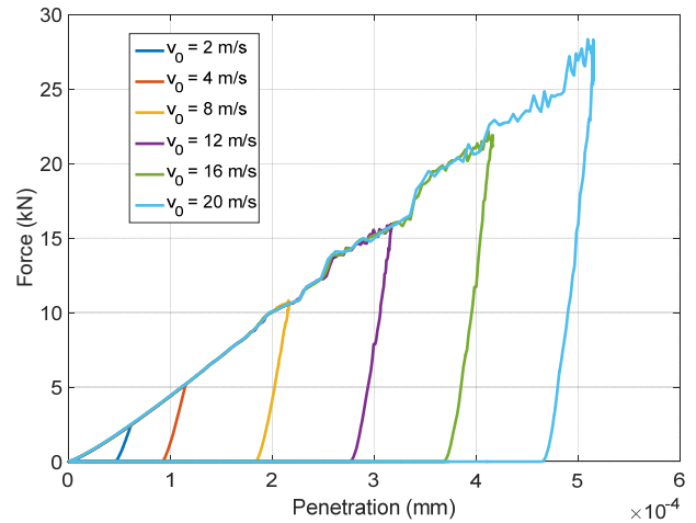
Fig. 8 Contact force versus penetration (plastic simulation)
