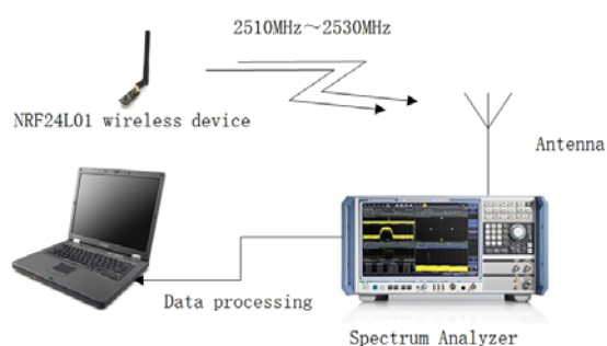
Fig. 4 Signal acquisition system
