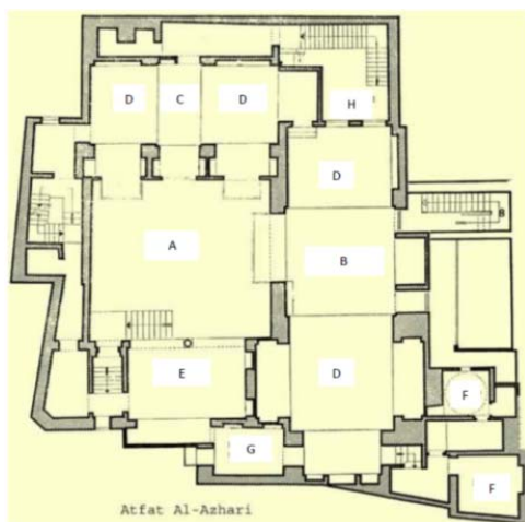
Fig. 2 House of Zainab Khatoun, Ground Floor Plan (1468 AD) [5]
