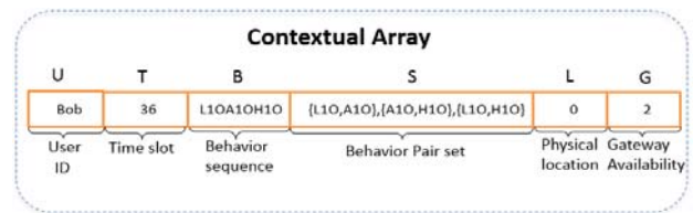
Fig. 5 Contextual array for a sample context
