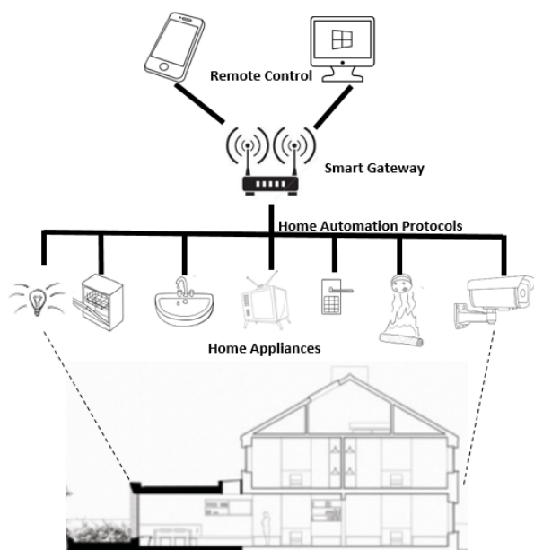
Fig. 4 Home Automation System Testbed
