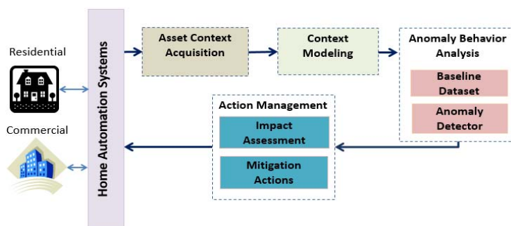
Fig. 2 CA-ABAS Architecture
