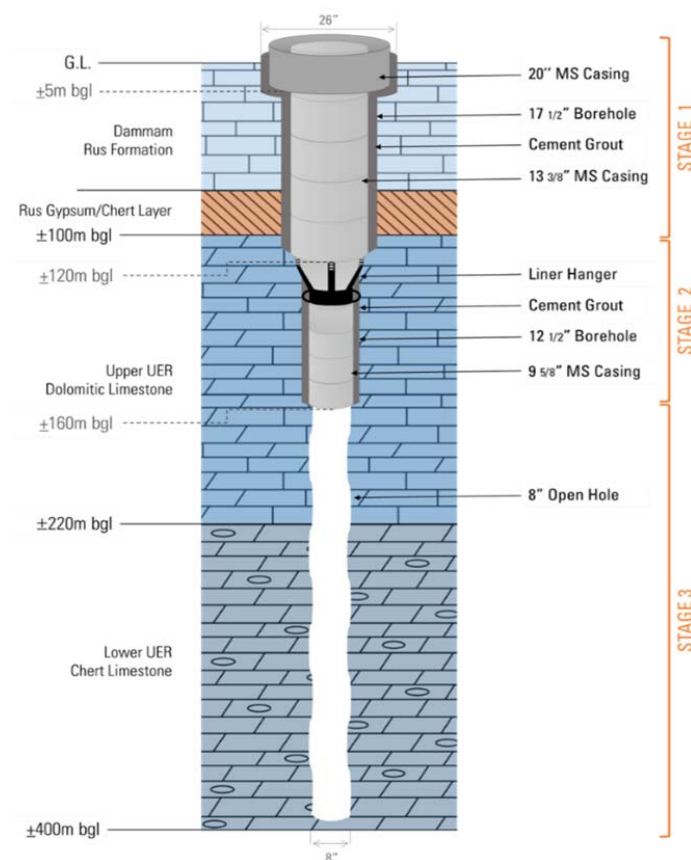
Fig. 10 Injection Well Completion – Stages 1 to 3
