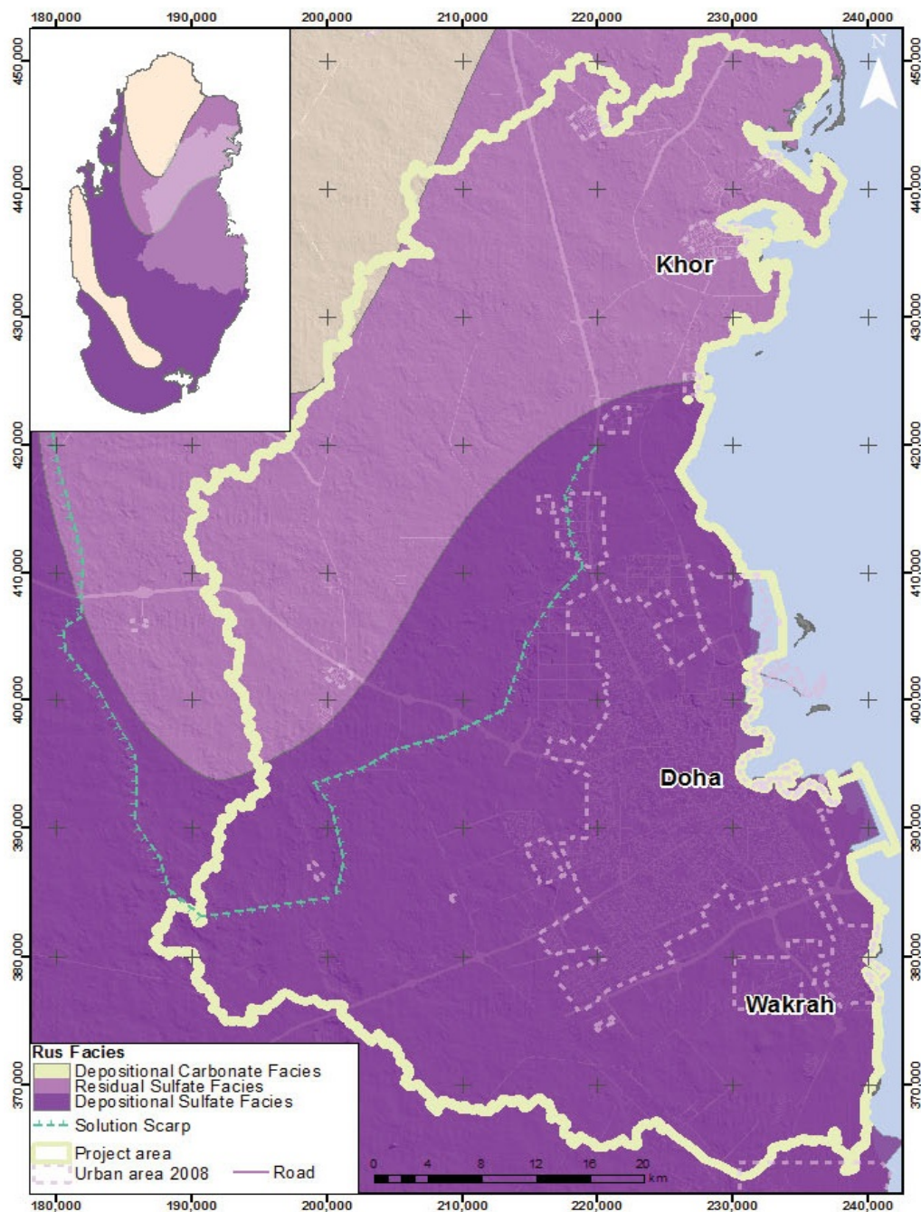
Fig. 5 Area of gypsum confinement in Doha Area [5]
