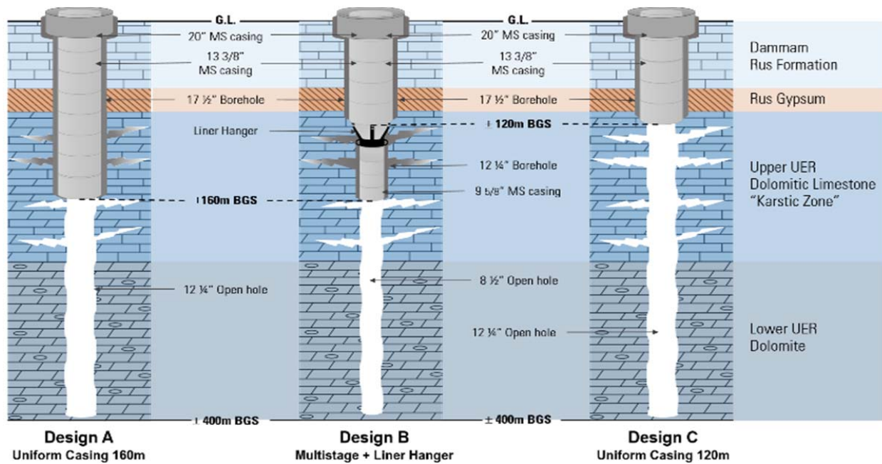
Fig. 11 Schematic of various injection well designs
