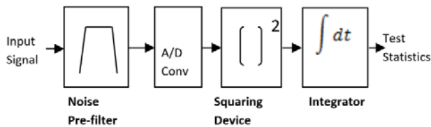
Fig. 2 Block diagram of the Energy Detector
