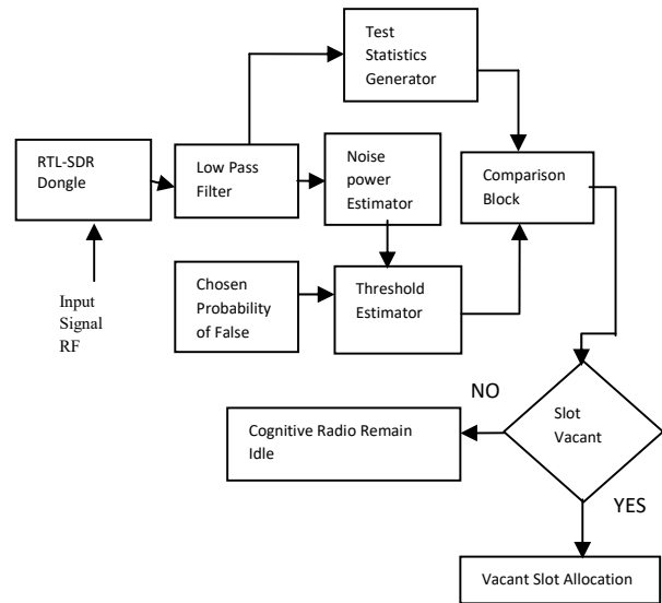
Fig. 3 Block diagram/Simulation set up of the Spectrum sensing and signal identification cognitive radio Simulink model
