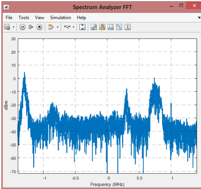
Fig. 6 Frequency spectrum for 94 - 94.9 MHz
