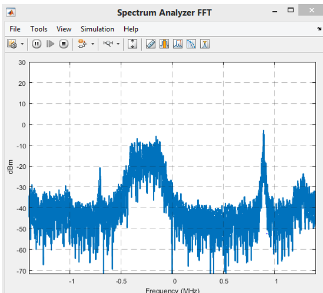
Fig. 7 Frequency spectrum for 95 - 95.9 MHz
