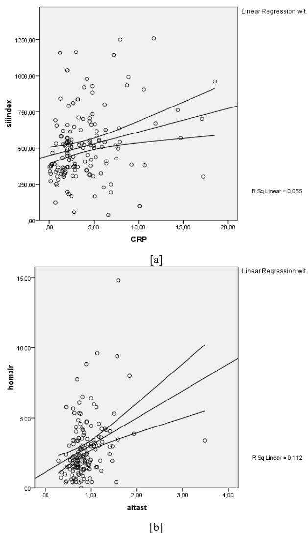
Fig. 1 Scatter plots of patient individual measurements for SII index versus CRP (a) and HOMA-IR versus ALT/AST (b) in MO children. Positive correlations are observed. Linear regression lines are displayed
