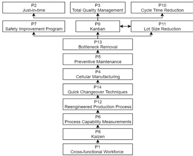
Fig. 2 ISM diagram
