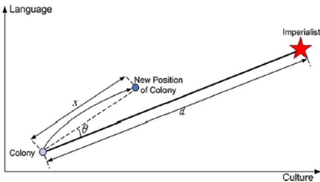
Fig. 3 Moving the colony towards the corresponding imperialist [24]
