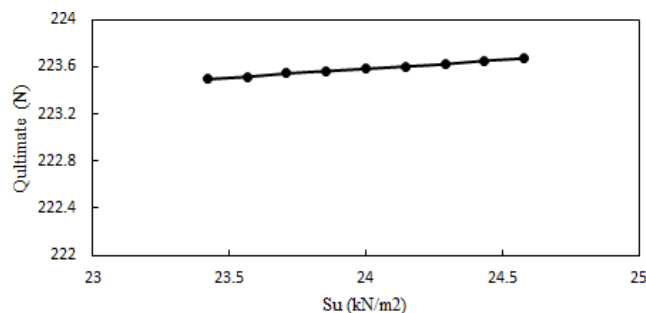
Fig. 16 Sensitivity results of ANN-ICA model to the undrained shear strength of soil
