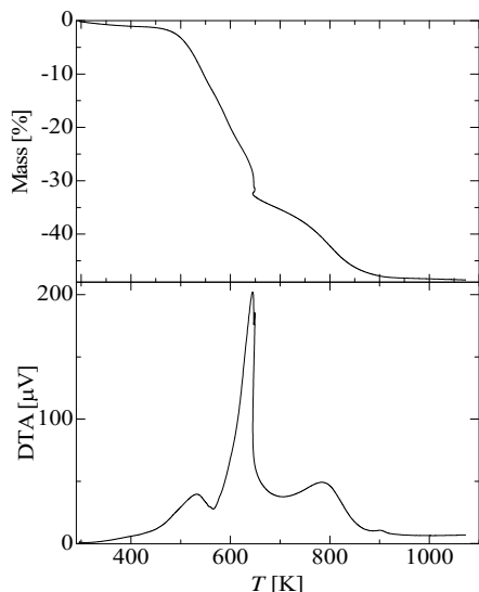
Fig. 5 TG/DTA curves of TOPEN impregnated adsorbent
