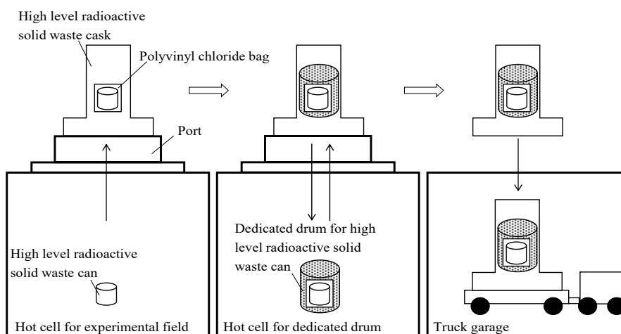
Fig. 6 Flow of transportation of high level radioactive solid waste can from the CPF to the 2nd HASWS in the TRP
