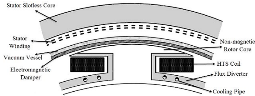
Fig. 1 General structure of new machine
